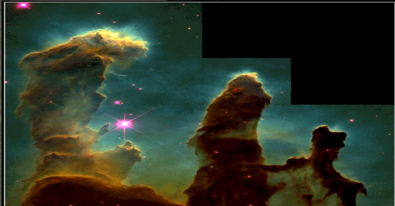
Gaseous Pillars - M16 HST - WFPC2 PRC95-44a - ST ScI OPO - November 2, 1995 J. Hester and P. Scowen (AZ State Univ.), NASA
